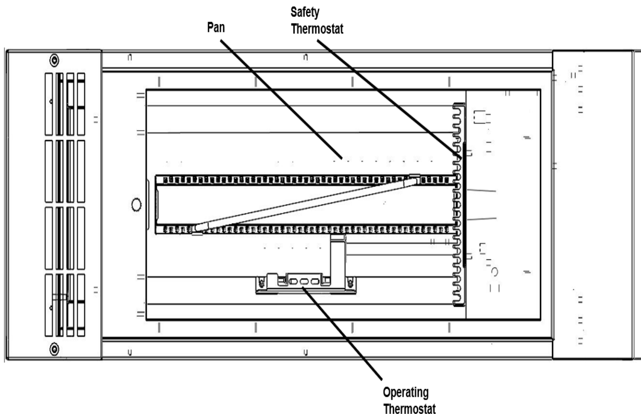
Location of Safety and Operating Thermostat Probes
