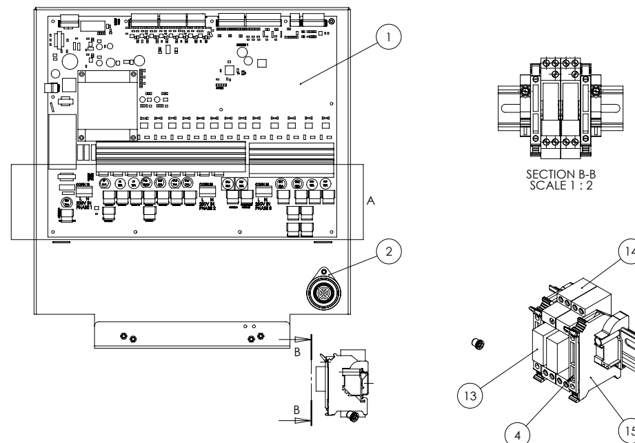
I/O BOARD DETAIL F2HH
