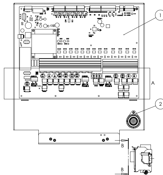
I/O BOARD DETAIL F2HH
