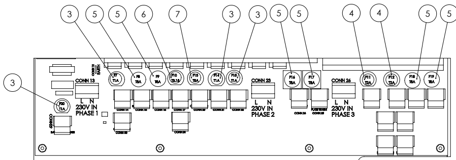
DETAIL A SCALE 1 : 1.5
